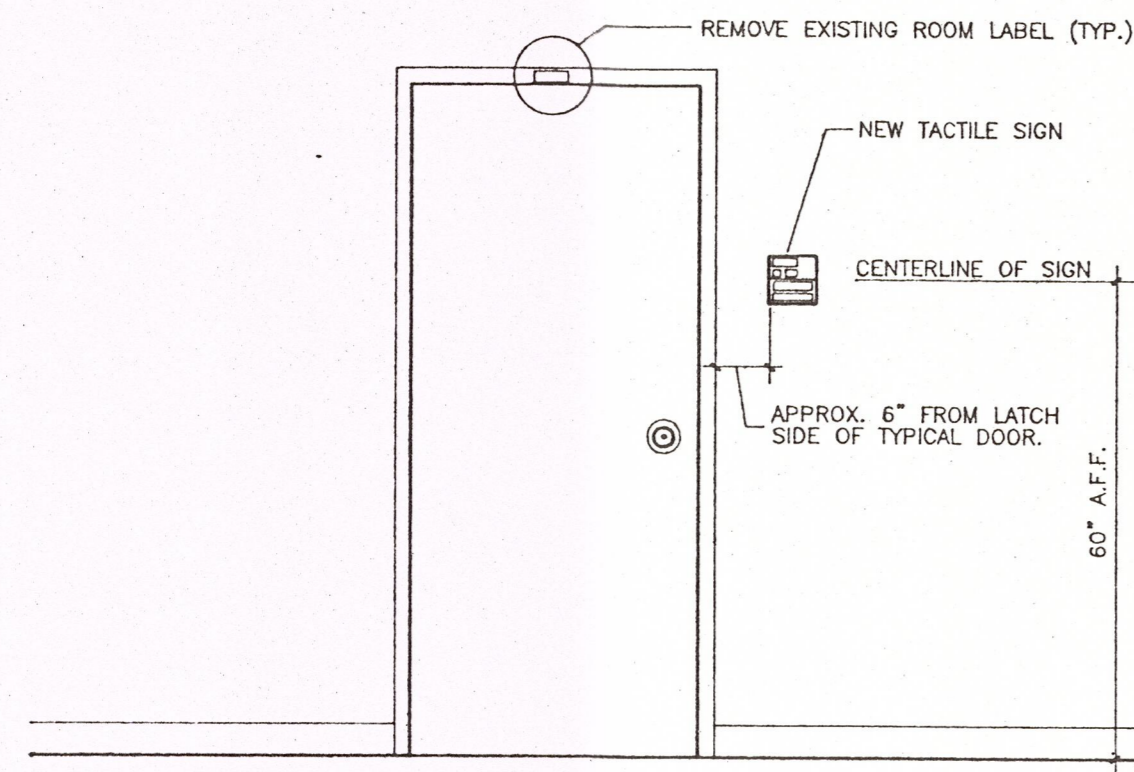
2 S3 TYPICAL TACTILE SIGNAGE LOCATION SCALE: 1/2" = 1'-0"
