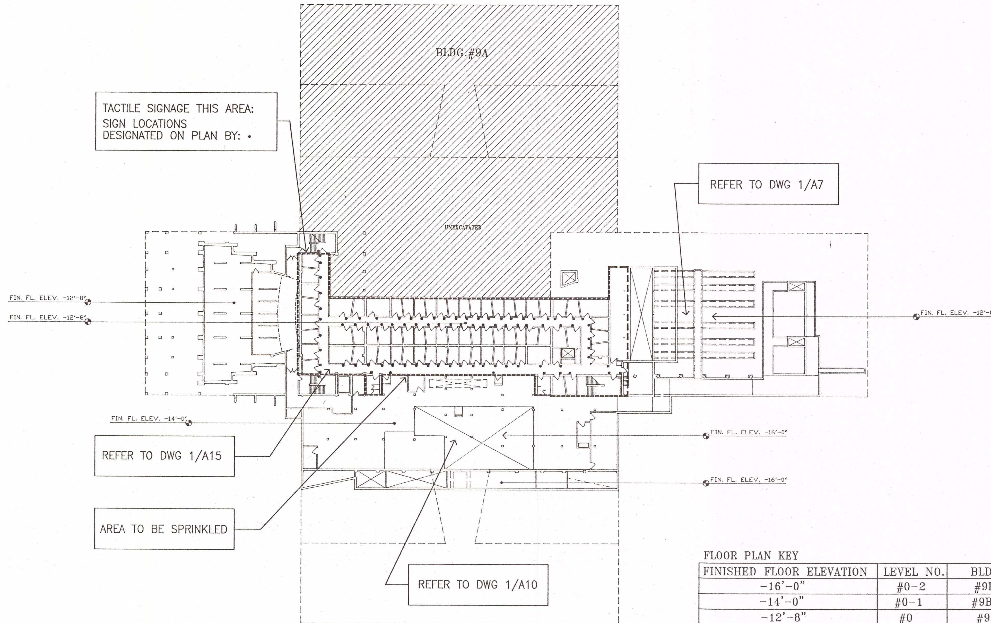
1 S3 CRANE MUSIC COMPLEX LEVEL - 0 SCALE: 1/32" = 1'-0"
