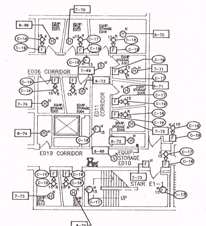
3 PARTIAL BASEMENT PLAN - LEVEL 0 SCALE: 1/16" = 1'-0"
