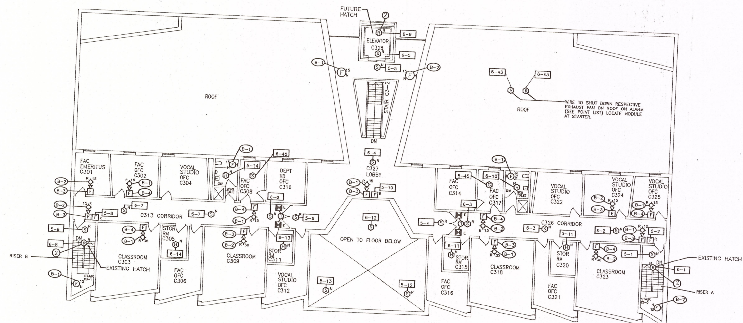
1 UPPER PLAN - LEVEL 3 A6 SCALE: 1/16" = 1'-0"
