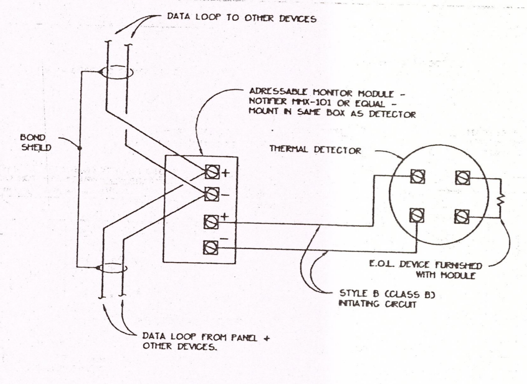
SINGLE DETECTORS (SPRINKLER FLOW + VALVE SUPERVISION, CAR PRESSURE SIMILAR TO VALVE TAMPER.)
