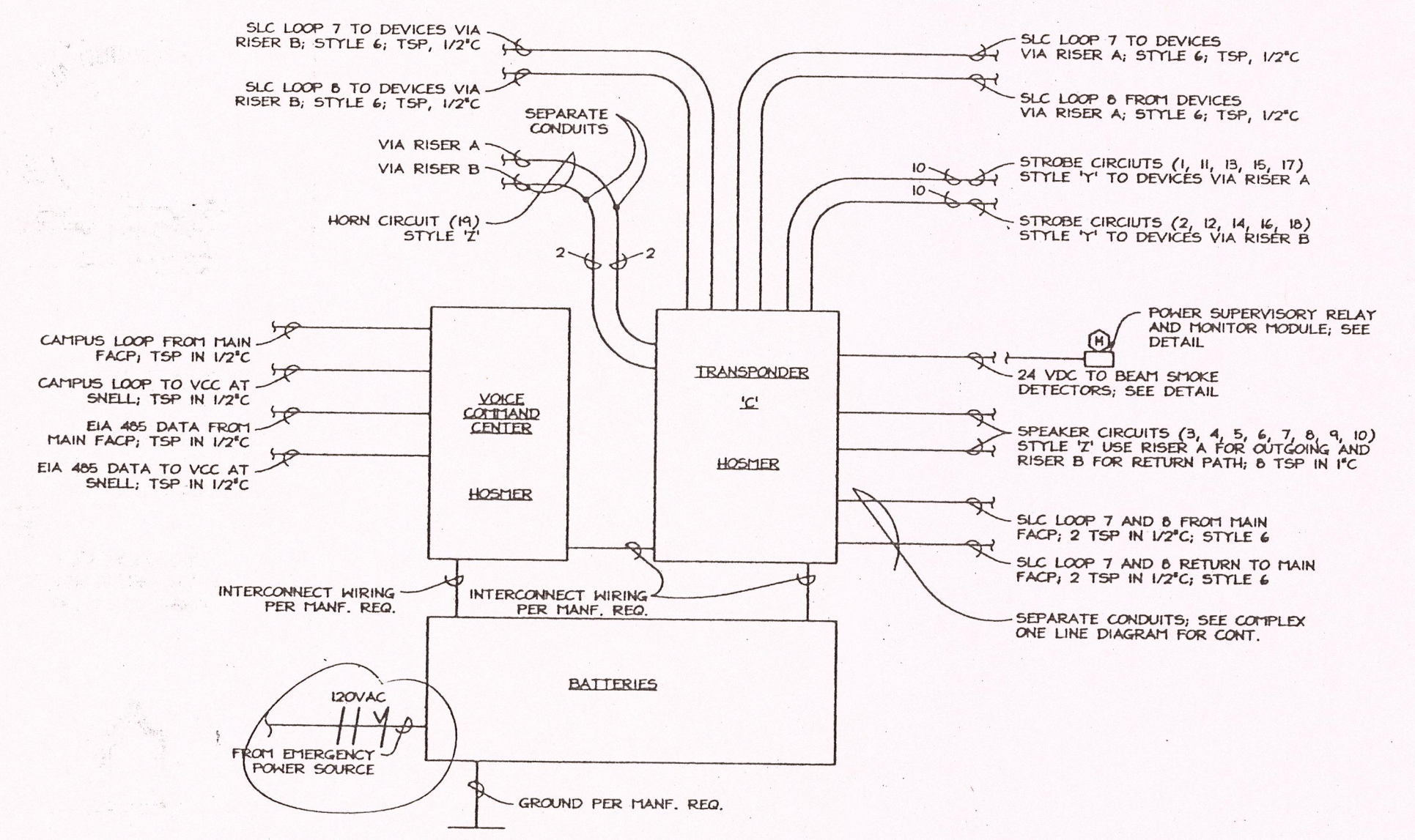
ONE-LINE DIAGRAM - CRANE MUSIC FIRE ALARM N.T.S.
