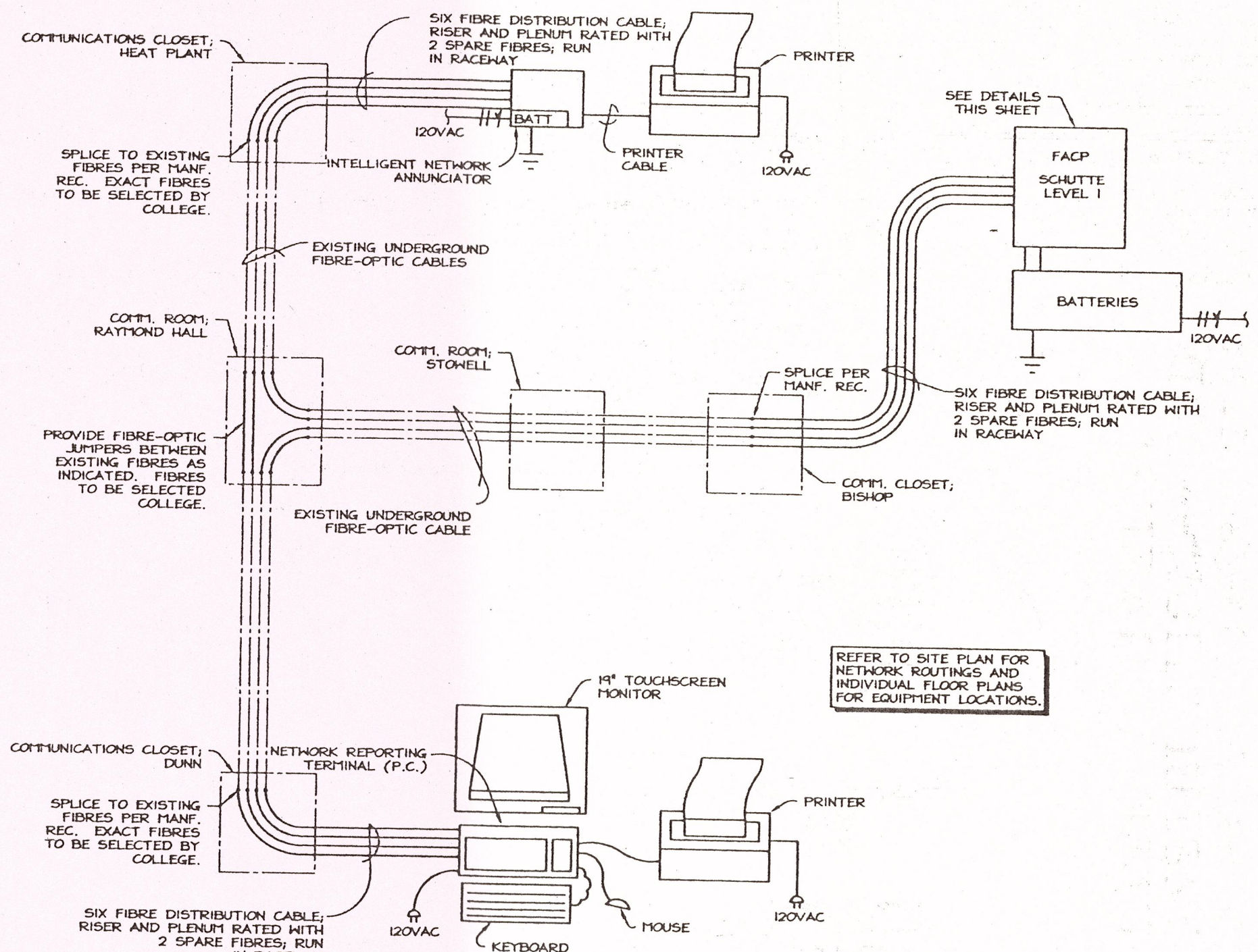
ONE-LINE DIAGRAM - FIRE ALARM NETWORK N.T.S.
