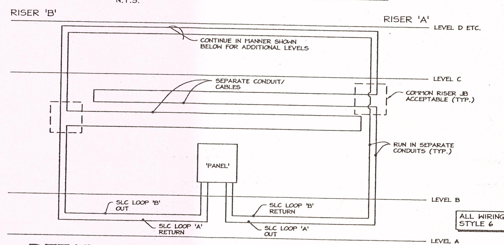
DETAIL - TYPICAL SLC LOOP RISER ROUTING N.T.S.
