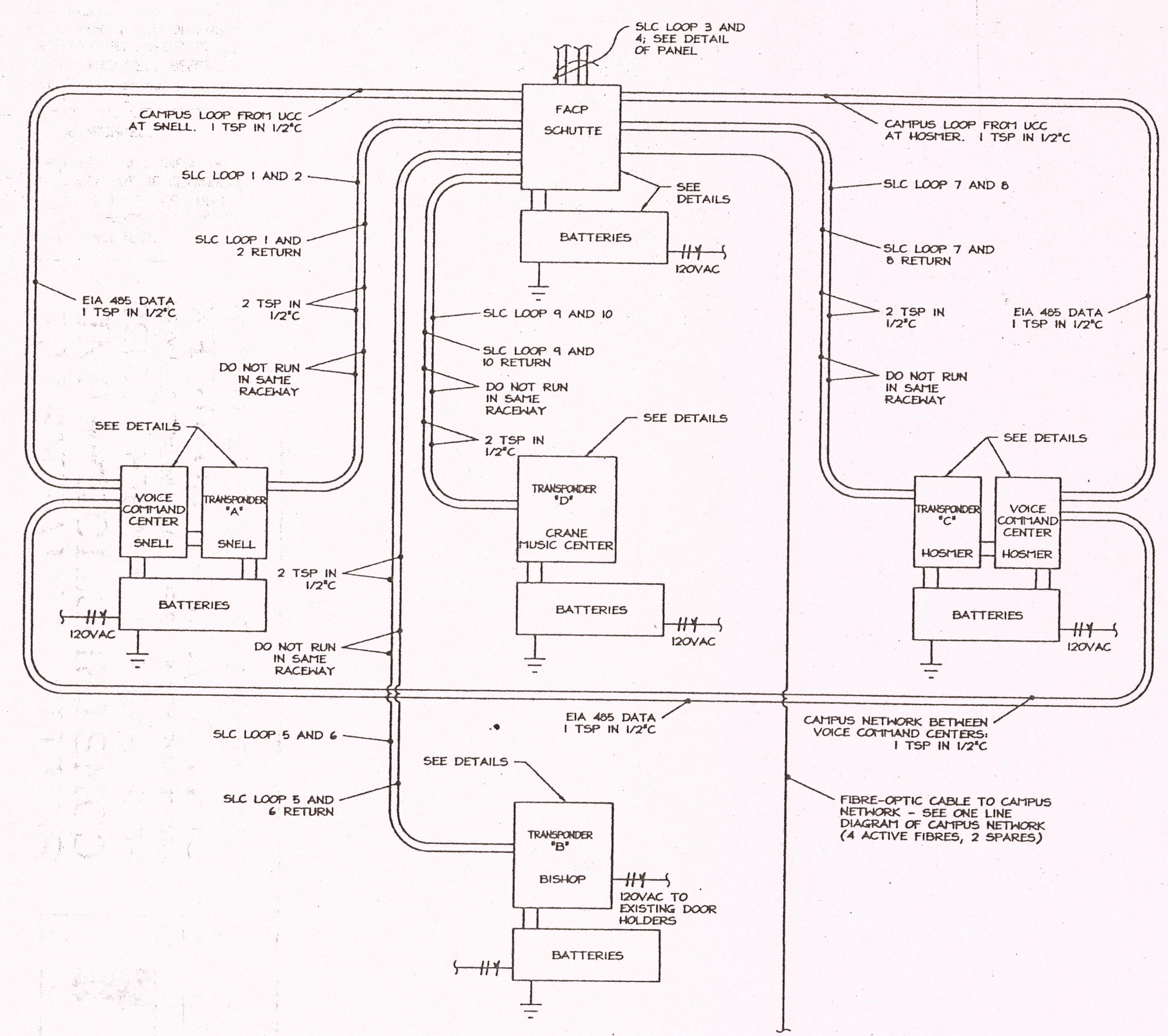
ONE-LINE DIAGRAM - CRANE MUSIC FIRE ALARM N.T.S.
