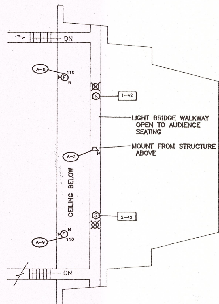
2 PARTIAL ATTIC PLAN - LEVEL 2 A2 SCALE: 1/16" = 1'-0"
