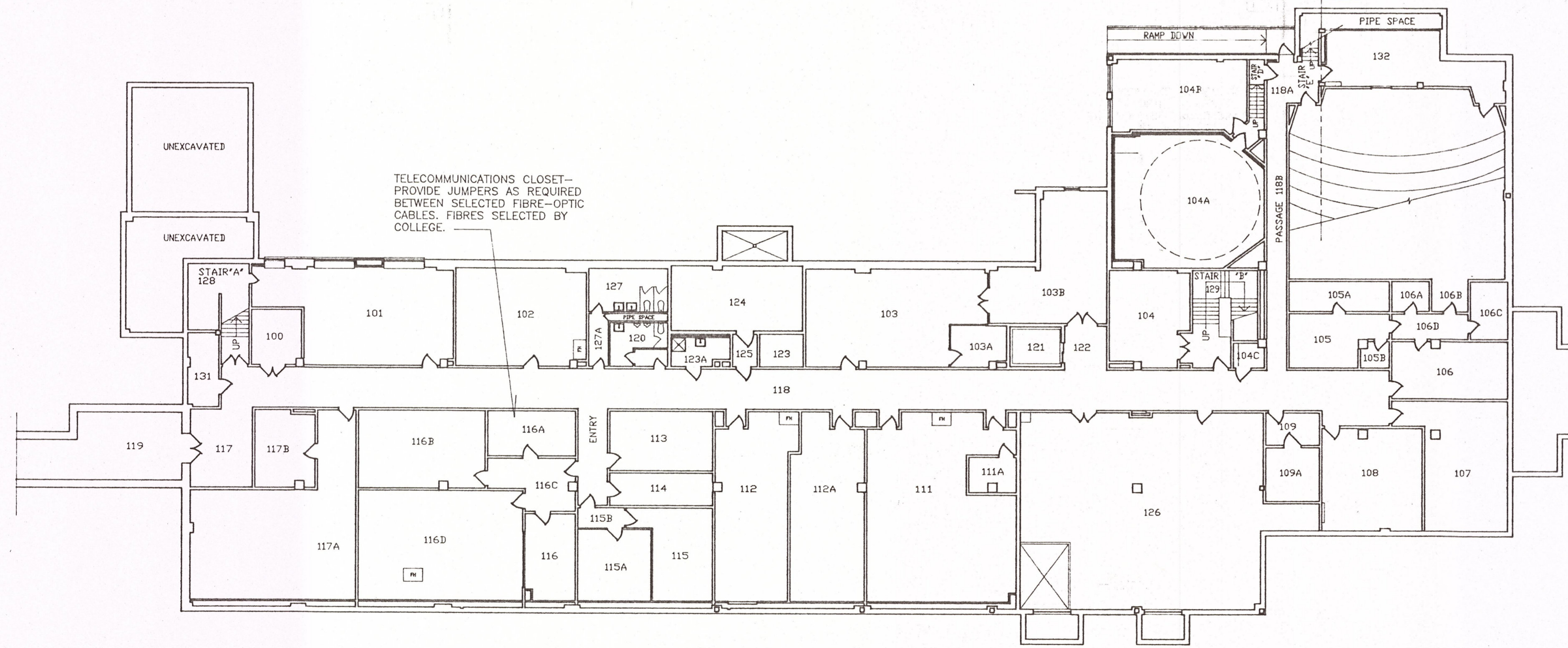
4 CELLAR PLAN - STOWELL HALL A16 NOT TO SCALE
