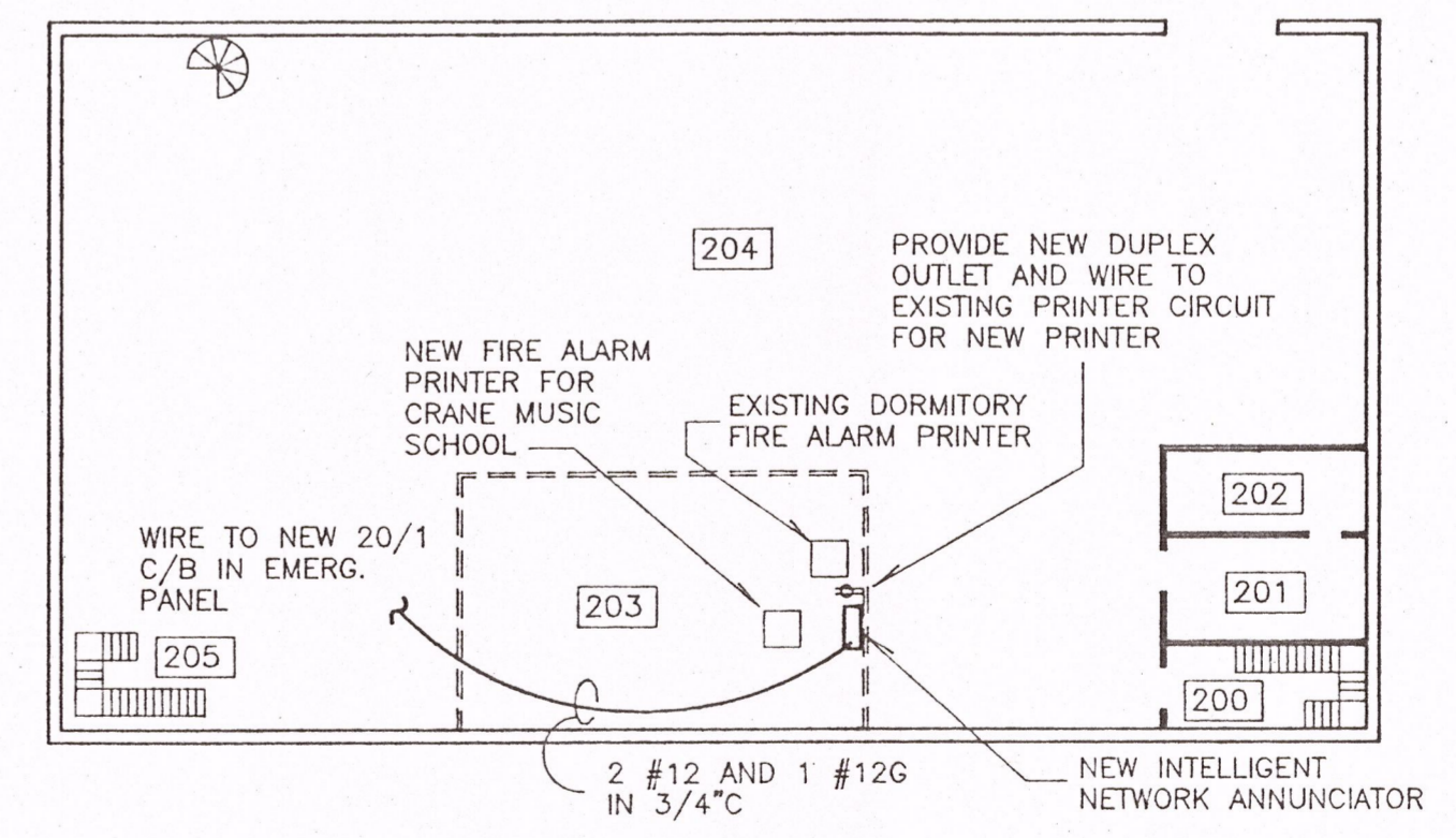
6 SECOND FLOOR - HEATING PLANT A16 NOT TO SCALE
