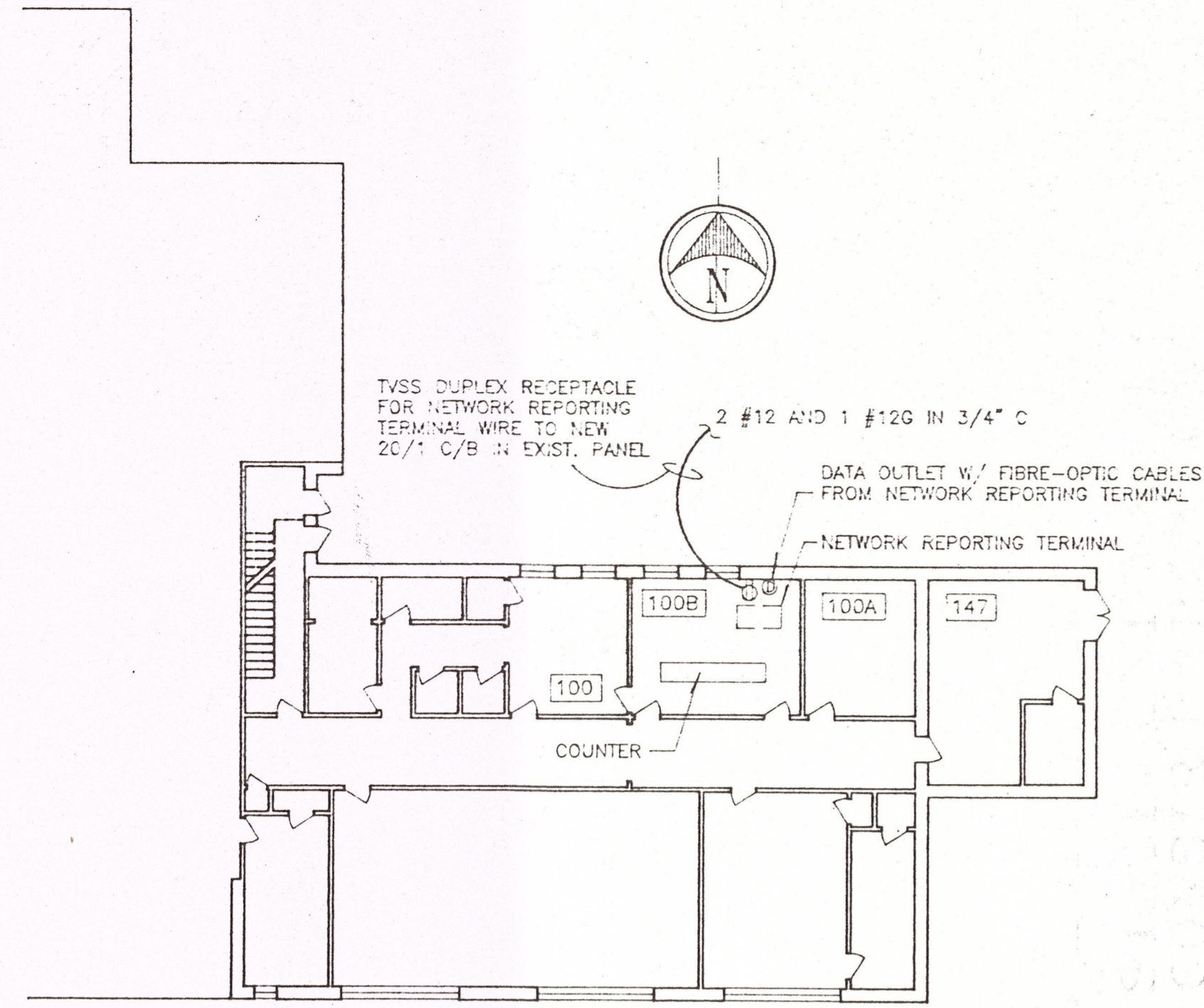
1 FIRST FLOOR - DUNN HALL A16 NOT TO SCALE
