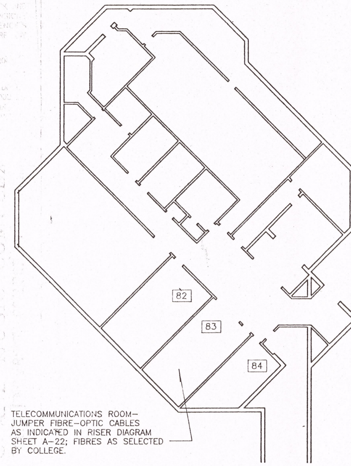
3 CELLAR PLAN - RAYMOND HALL A16 NOT TO SCALE
