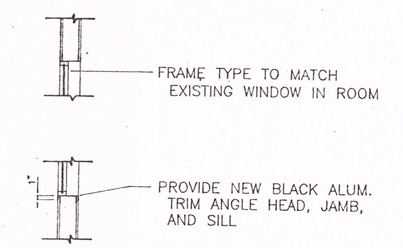
10 FIXED WINDOW SECTION A12 SCALE: 1/4" = 1'-0"
