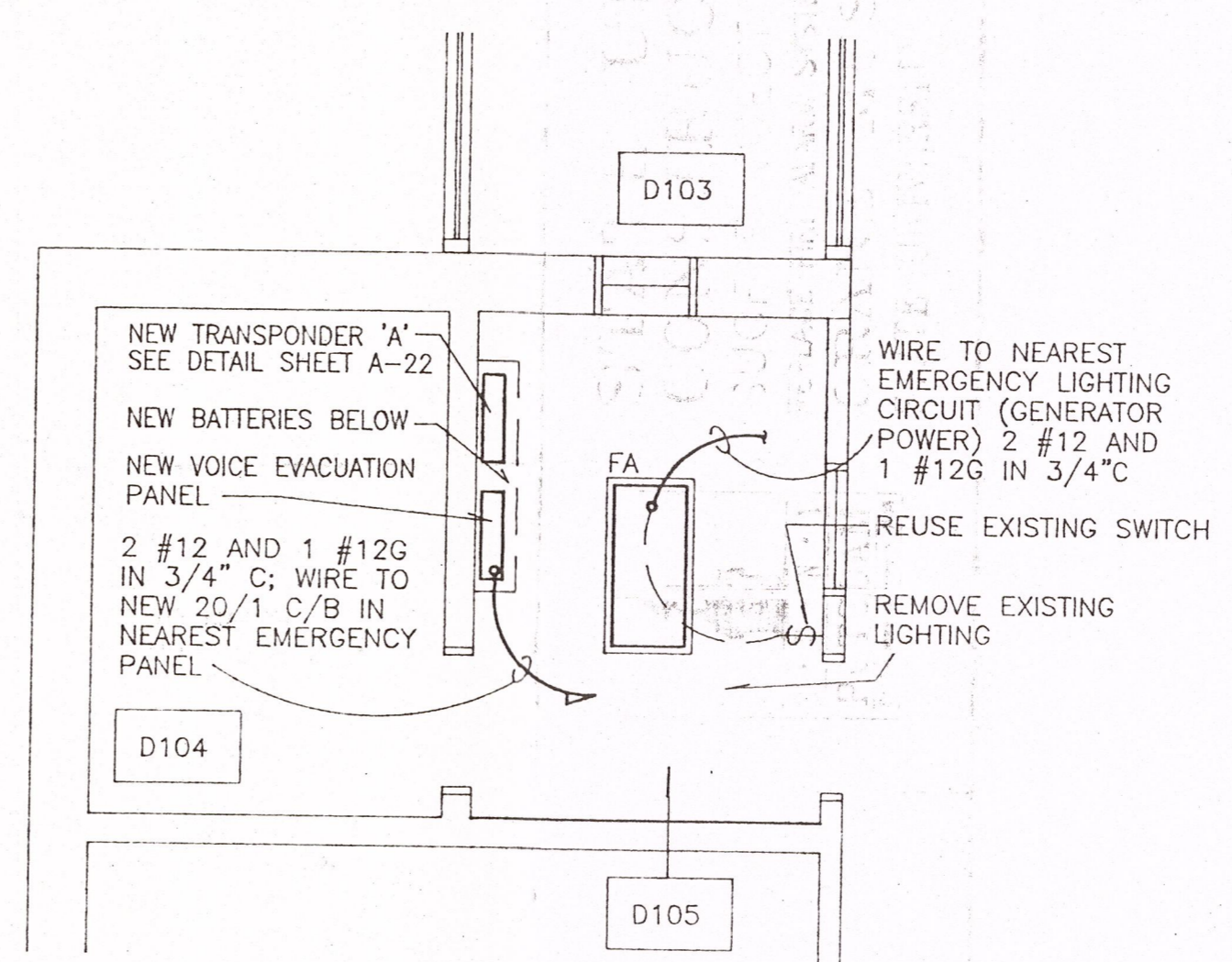
9 PARTIAL ELECTRICAL PLAN A12 SCALE: 1/4" = 1'-0"
