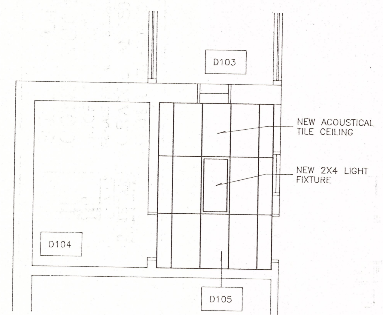
8 PARTIAL REFLECTED CEILING PLAN A12 SCALE: 1/4" = 1'-0"
