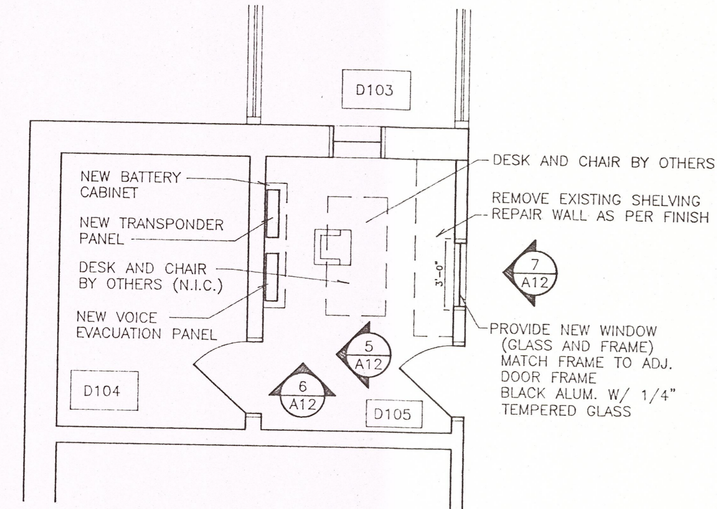
4 PARTIAL PLAN A12 SCALE: 1/4" = 1'-0"
