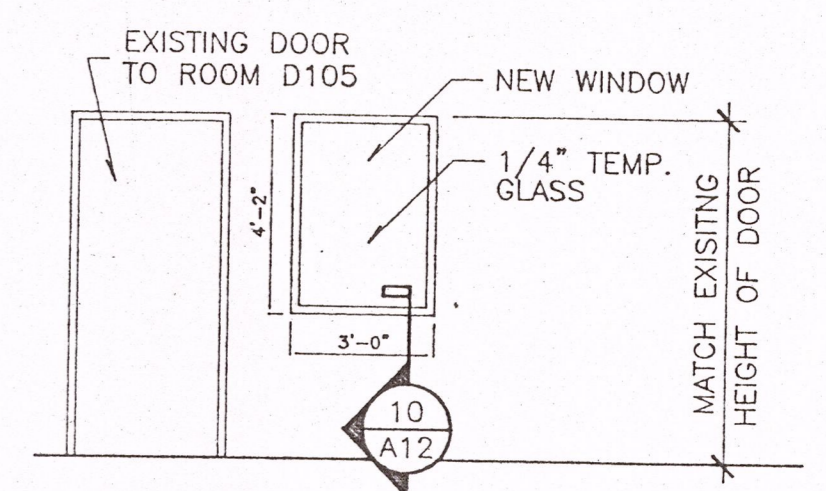
7 INTERIOR ELEVATION A12 SCALE: 1/4" = 1'-0"
