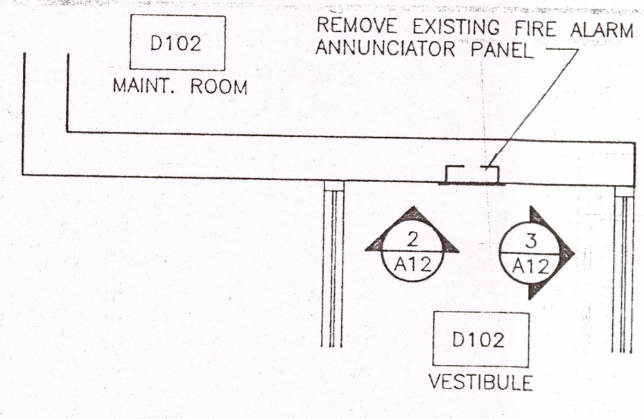
1 PARTIAL PLAN A12 SCALE: 1/4" = 1'-0"
