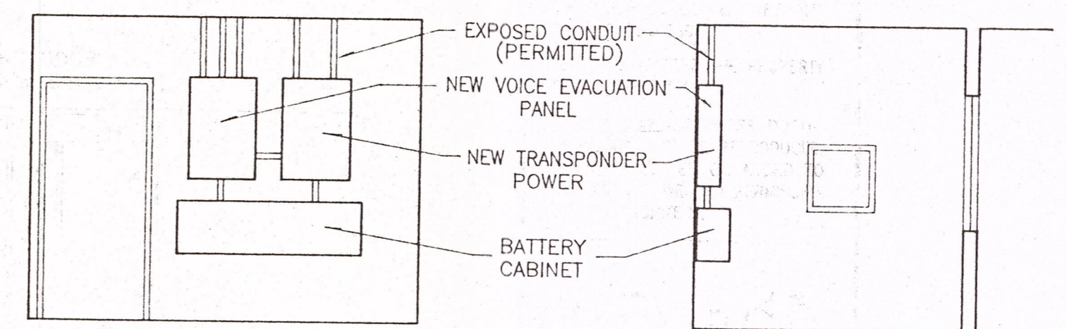
5 INTERIOR ELEVATION A12 SCALE: 1/4" = 1'-0"
