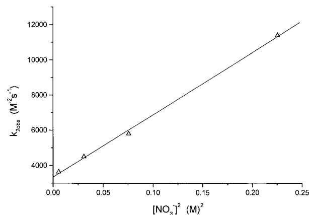
Figure 4. Plot of k_{\text{obs}} against [\text{NO}_3^-]^2 ; intercept, 3.4(\pm 0.5) \times 10^3 \text{ M}^{-2} \text{ s}^{-1} ; slope, 3.5(\pm 0.5) \times 10^4 \text{ M}^{-4} \text{ s}^{-1} , r = 0.99907 .
