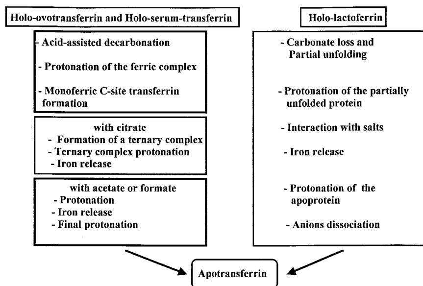
Figure 5. A simplified approach to the mechanisms of iron release by serum transferrin, ovotransferrin and lactoferrin at \mu \leq 0.5 .
