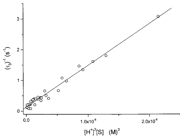
Figure 2. Plot of (\tau_3)^{-1} against [H^+]^2[S]^n at 25(\pm 0.5)^\circ\text{C} for 2\ \mu\text{M} \leq c_1 \leq 50\ \mu\text{M} , with n=1 and 18.75\ \text{mM} \leq [S] = [\text{SO}_4^{2-}] \leq 120\ \text{mM} ; intercept, 0.13(\pm 0.03)\ \text{s}^{-1} ; slope, 1.35(\pm 0.15) \times 10^6\ \text{M}^{-3}\ \text{s}^{-1} and r = 0.98964 .
