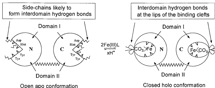
Figure 6. Schematic view of the modifications in the conformation of transferrin when it goes from an open apotransferrin to a closed holotransferrin with the occurrence of interdomain H-bonds at the lips of the Fe(III) binding clefts. x is the number of protons lost during iron uptake and \text{Fe(III)L} is the iron donor chelate (Bou Abdallah & El Hage Chahine, 1998).
