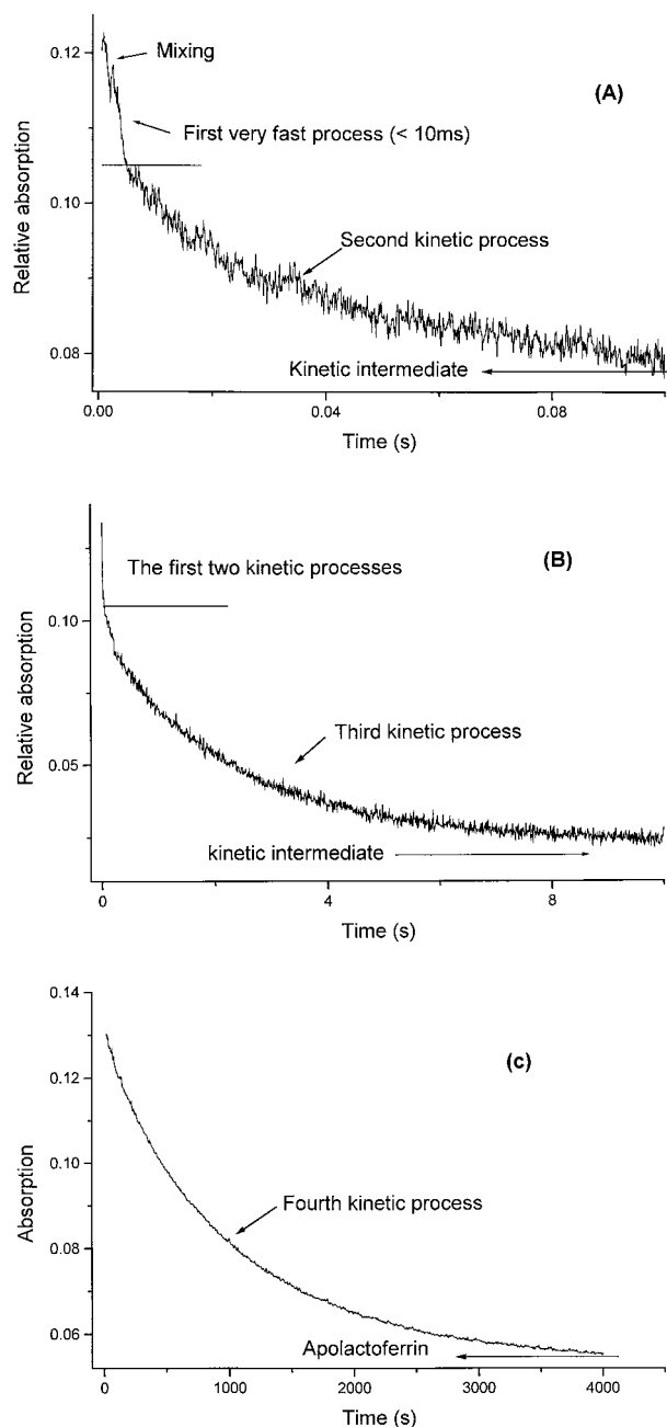
Figure 1. Fluorescence and absorption variation with time, when a solution of bovine hololactoferrin is submitted to a fast pH-jump from neutral to acidic media with \lambda = 465 nm for absorption and an excitation wavelength \lambda_{\text{ex}} = 280 nm for emission at 25(\pm 0.5)^\circ\text{C} . (a) to (c) Multiexponential decreases of absorption recorded on three different time-scales in the presence of (a) 180 mM KBr at pH 2.54, (b) 30 mM NaBr at pH 2.14 and (c) 150 mM KCl at pH 3.16, with c_1 = 50 \mu\text{M} .
